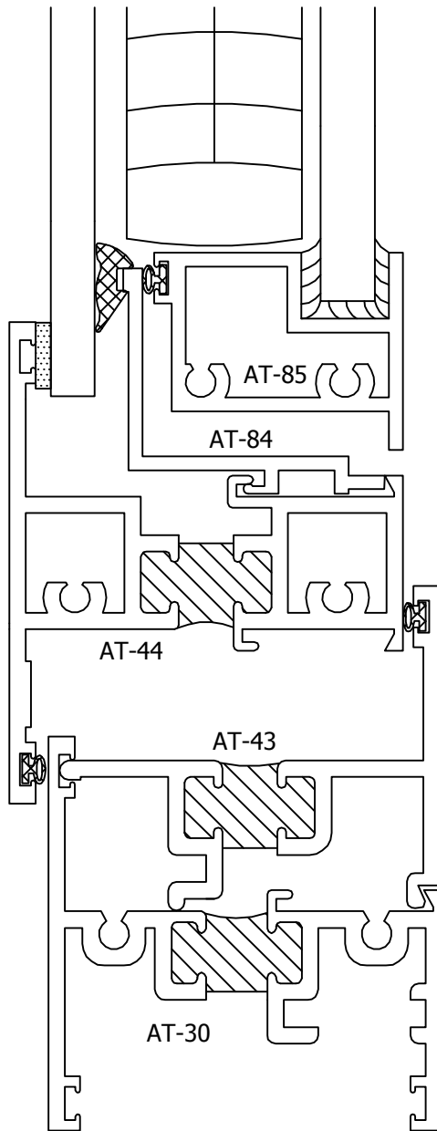
20 SILL @ VENT
