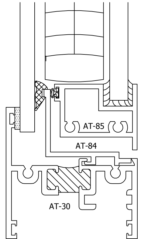
21 SILL @ FIXED
