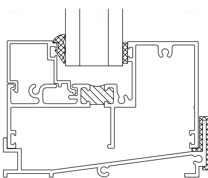
⑨ FIXED WINDOW SILL
