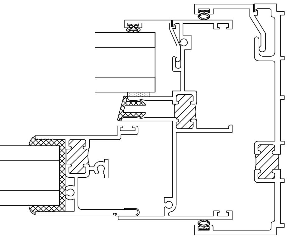
11 HEAD WITH COMP CHANNEL
