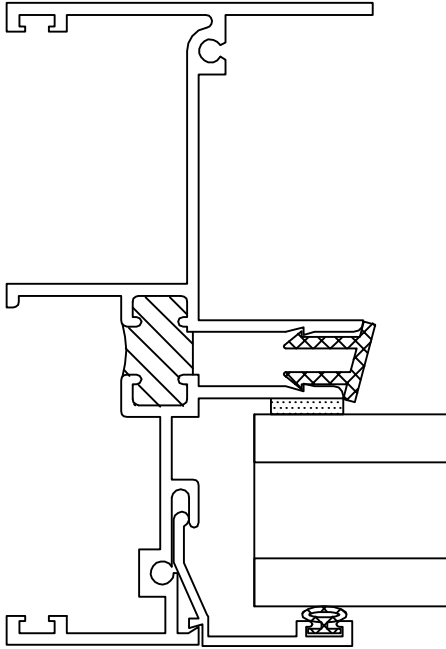
3 JAMB @ FIXED
